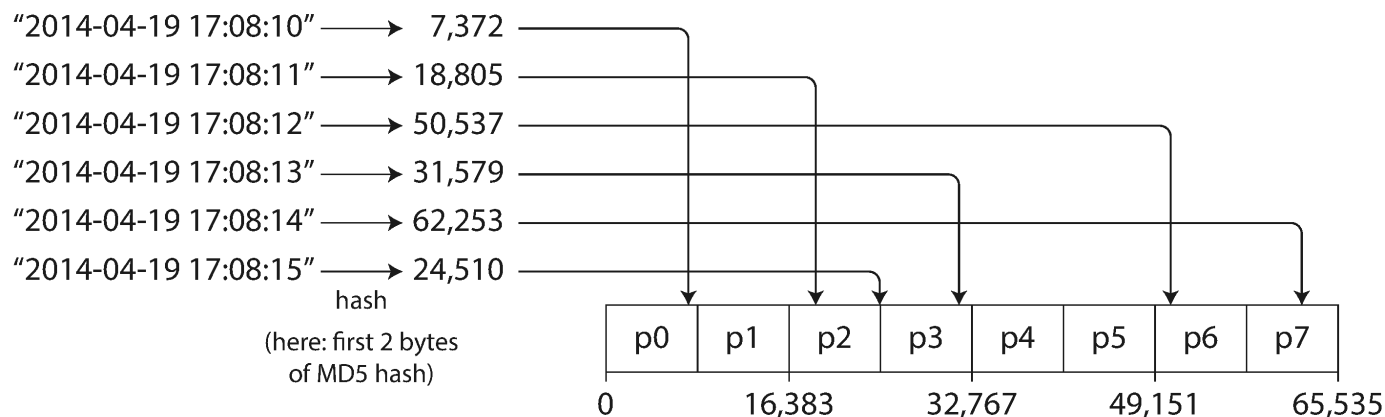
Figure 6-3. Partitioning by hash of key.
