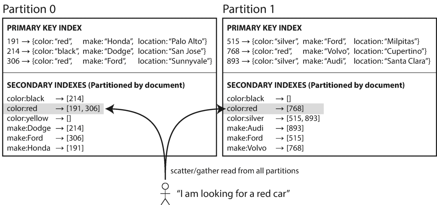
Figure 6-4. Partitioning secondary indexes by document.
