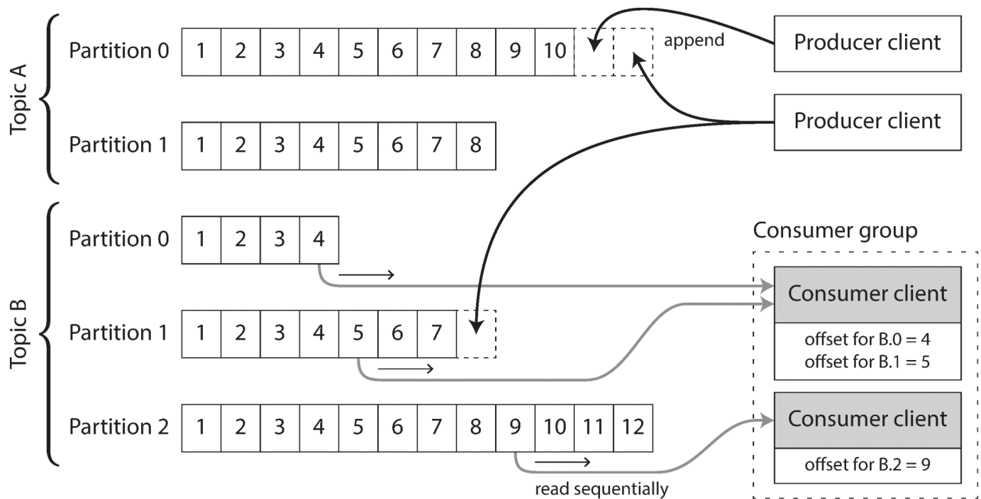
Figure 11-3. Producers send messages by appending them to a topic-partition file, and consumers read these files sequentially.
