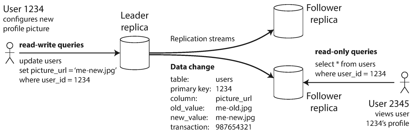
Figure 5-1. Leader-based (master–slave) replication.
