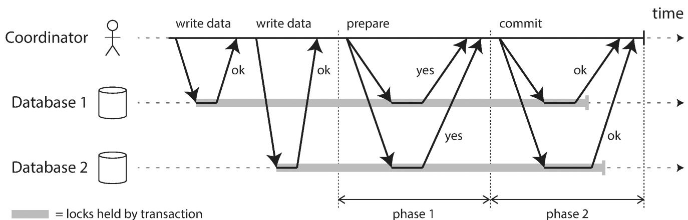
Figure 9-9. A successful execution of two-phase commit (2PC).
