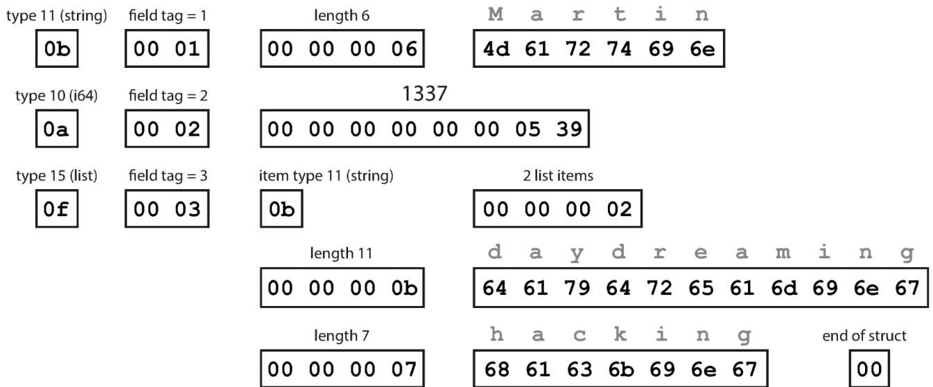
Figure 4-2. Example record encoded using Thrift's BinaryProtocol.
