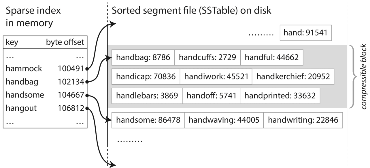
Figure 3-5. An SSTable with an in-memory index.
