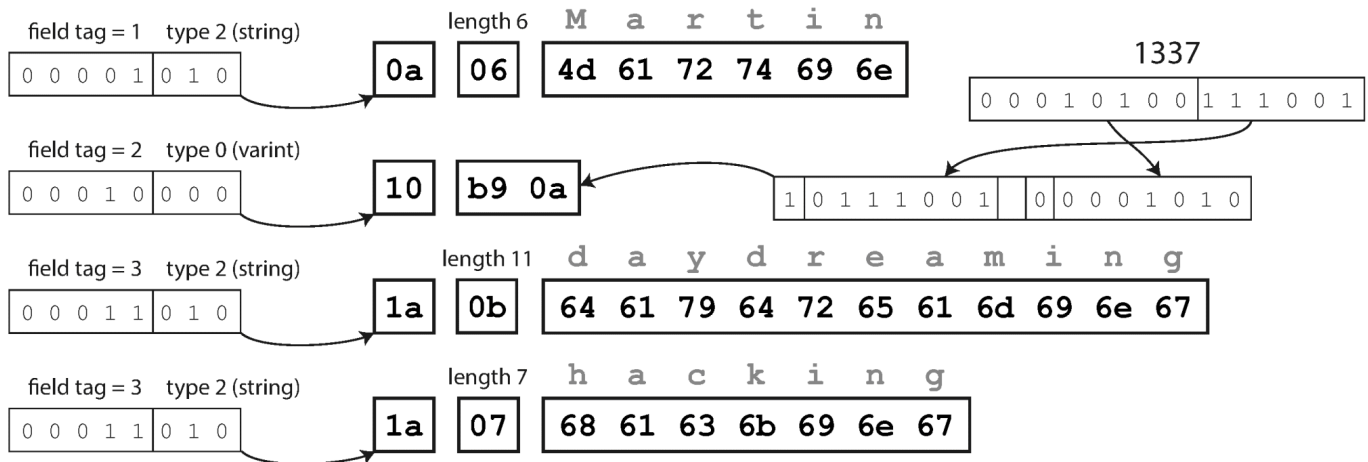
Figure 4-4. Example record encoded using Protocol Buffers.
