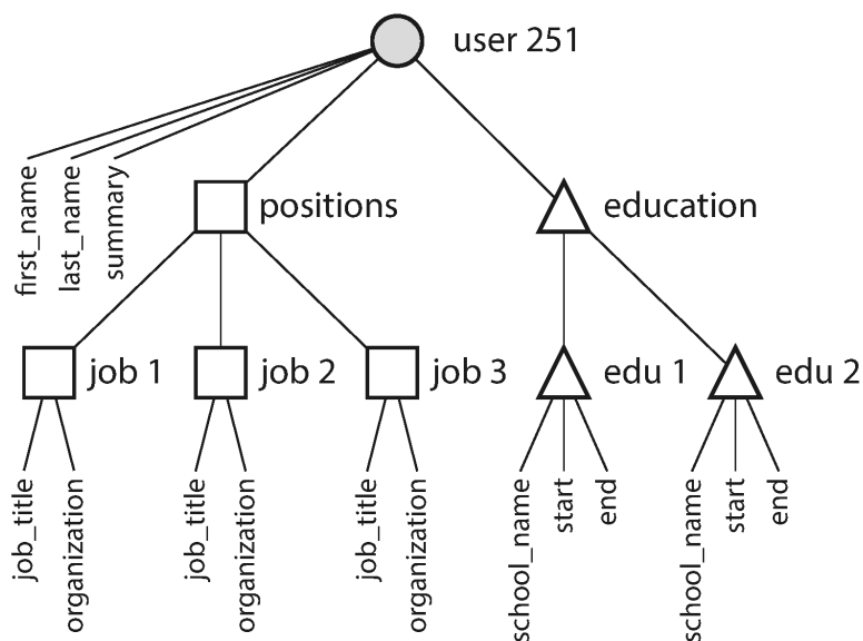
Figure 2-2. One-to-many relationships forming a tree structure.
