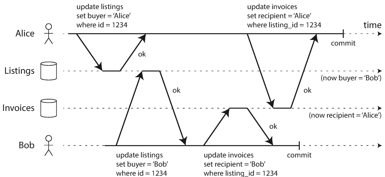
Figure 7-5. With dirty writes, conflicting writes from different transactions can be mixed up.
