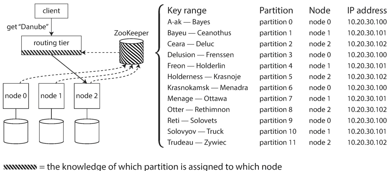
Figure 6-8. Using ZooKeeper to keep track of assignment of partitions to nodes.
