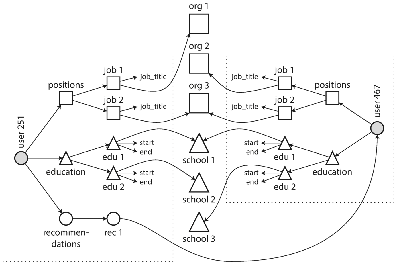
Figure 2-4. Extending résumés with many-to-many relationships.
