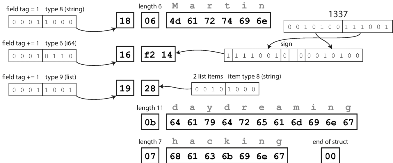
Figure 4-3. Example record encoded using Thrift's CompactProtocol.
