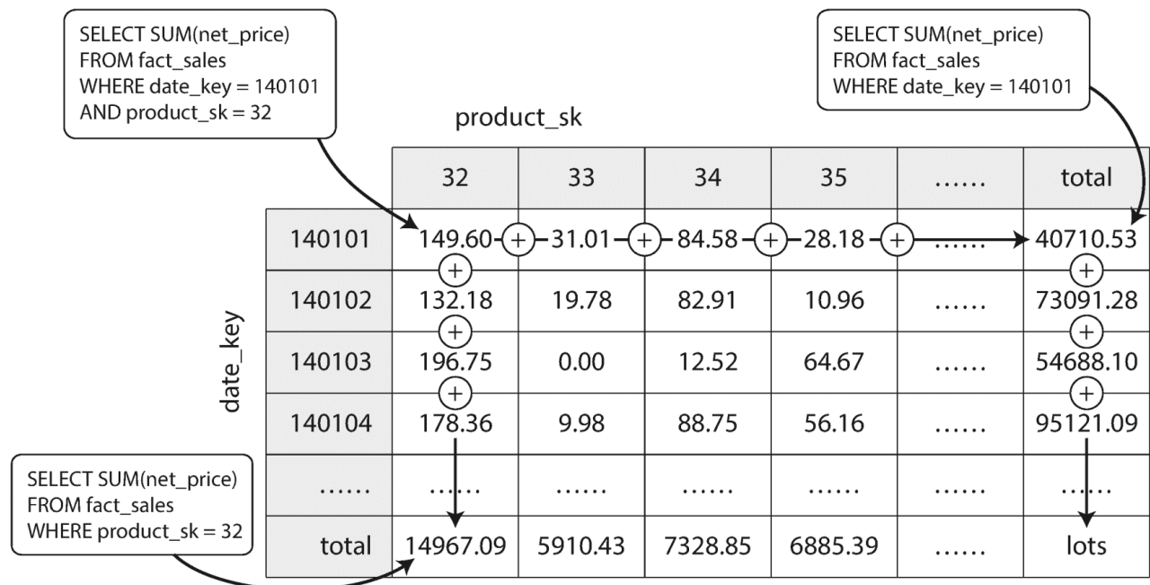
Figure 3-12. Two dimensions of a data cube, aggregating data by summing.
