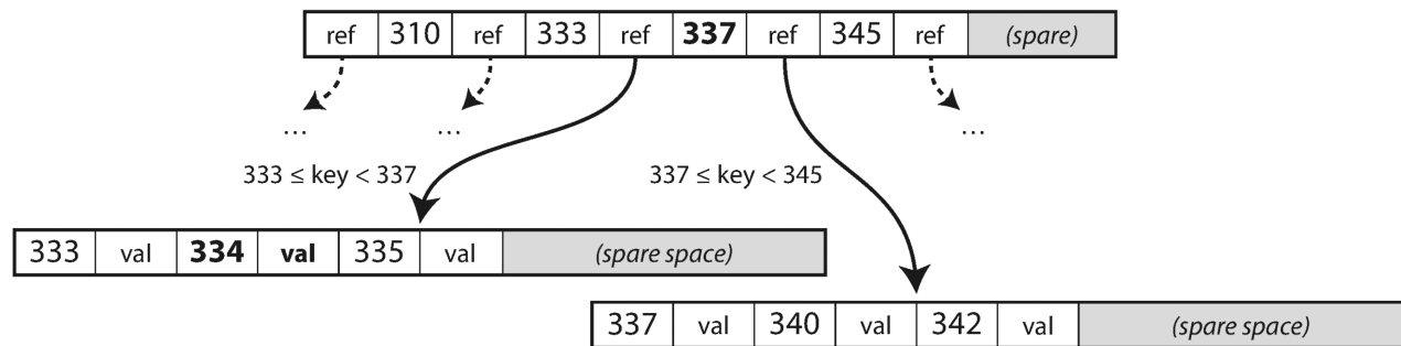
Figure 3-7. Growing a B-tree by splitting a page.
