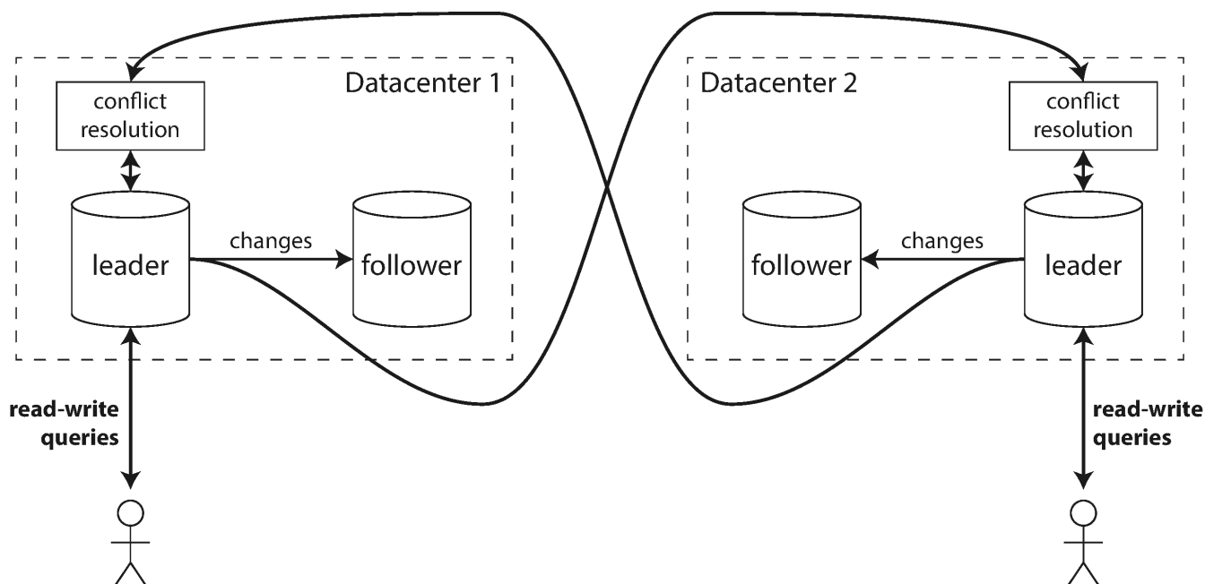
Figure 5-6. Multi-leader replication across multiple datacenters.
