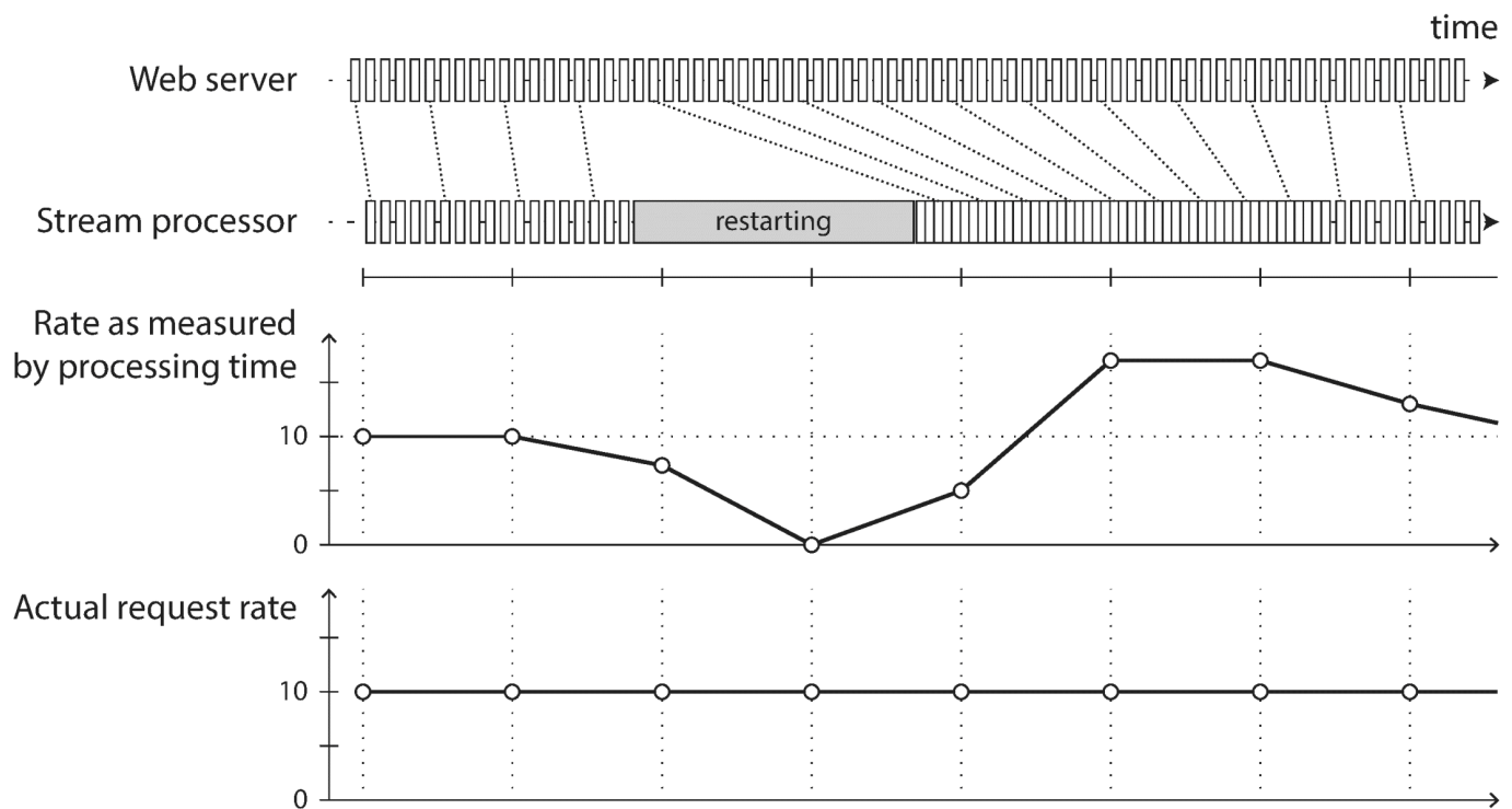
Figure 11-7. Windowing by processing time introduces artifacts due to variations in processing rate.
