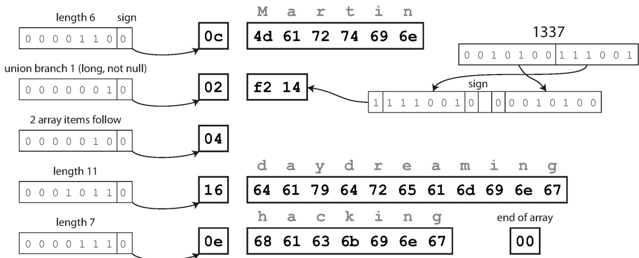
Figure 4-5. Example record encoded using Avro.
