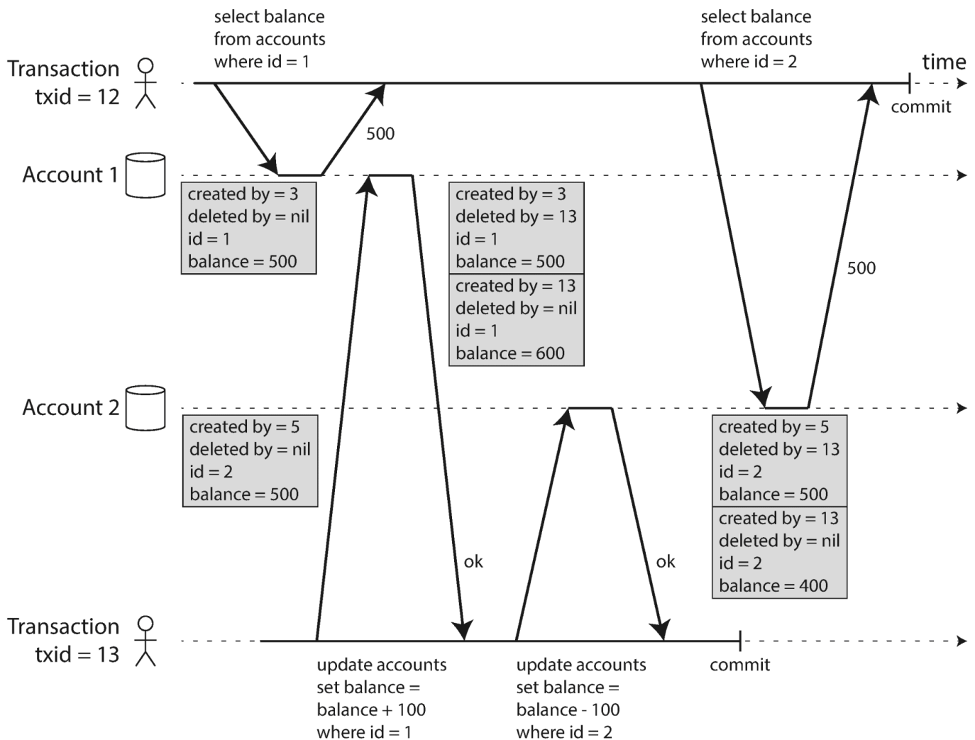
Figure 7-7. Implementing snapshot isolation using multi-version objects.
