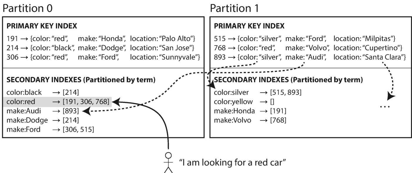
Figure 6-5. Partitioning secondary indexes by term.
